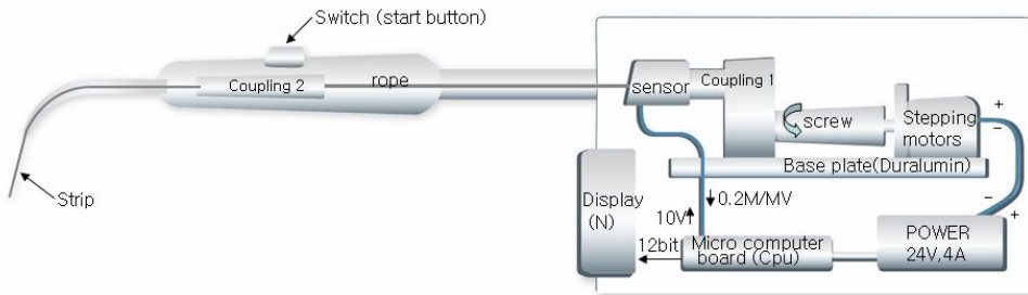
Fig. 2. Diagram of the measuring system(from Choi 12) ).
