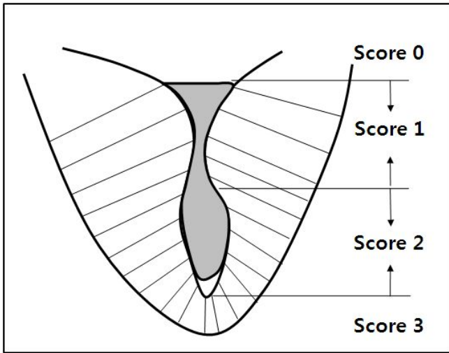
Fig. 2. Schematic diagram of the cross-sectioned specimen for measuring microleakage and sealant penetration depth
