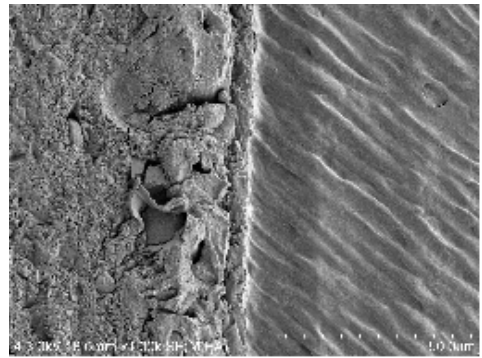
Fig 4. SEM photograph showing the close adaptation at the dentin-resin cement interface produced by Group 3 (All-Bond SE).
