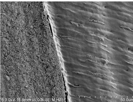
Fig 5. SEM photograph showing the gap at the dentin-resin cement interface produced by Group 4 (Isodan + One-step).
