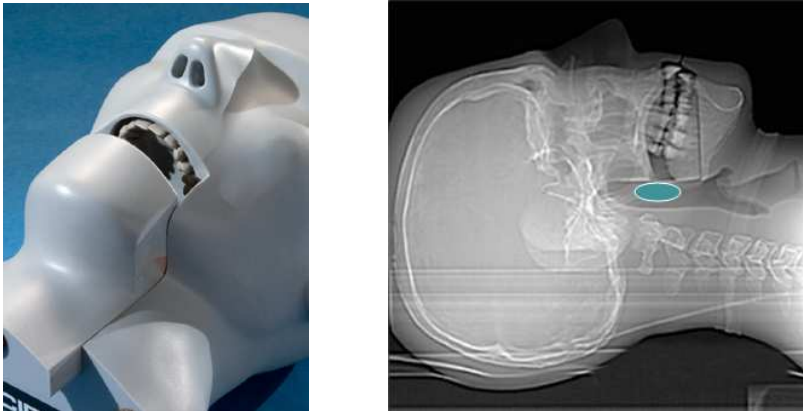
Fig. 2. Dental head phantom and x-ray image with water vinyl envelope in the esophagus
