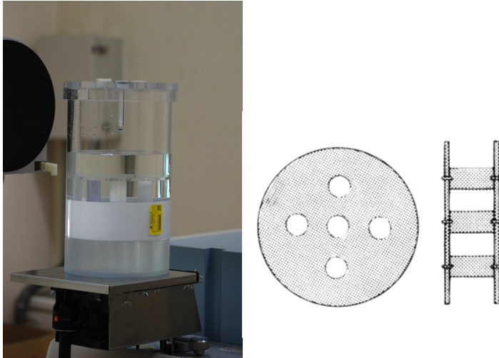
Fig. 1. AAPM phantom for the CT Number Insert(block) consists of five pins, each 1" in diameter, fabricated of the following materials: Density ( \text{gcm}^{-3} ) : Acrylic; 1.19, Polystyrene; 1.05, Polycarbonate; 1.20, Polyethylene; 0.95, Nylon; 1.10, Teflon; 2.21
