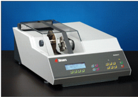
Fig. 2. High speed precision cut-off(Accutom-5, Struers, Denmark).
