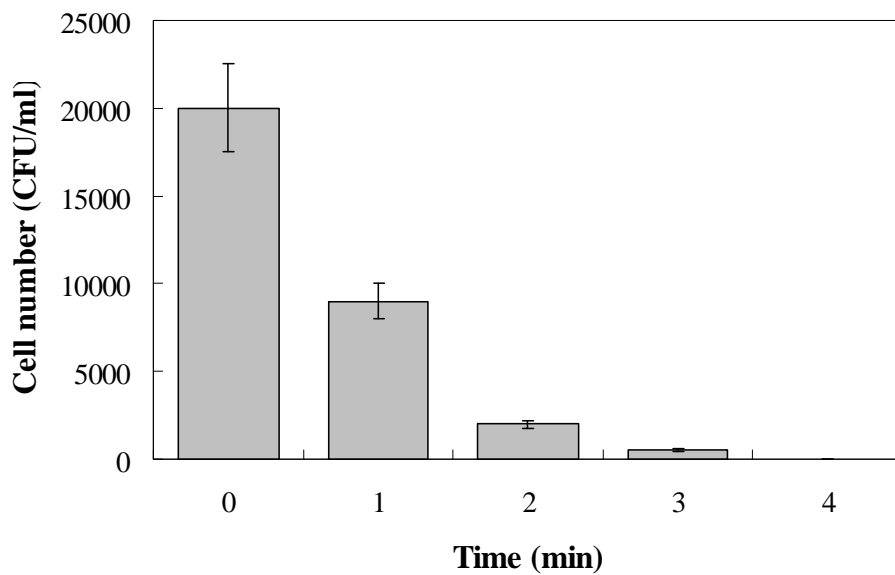
Figure 3. Bactericidal activity of S. sobrinus as a function of reaction time at propolis concentration 100 µg/ml.
