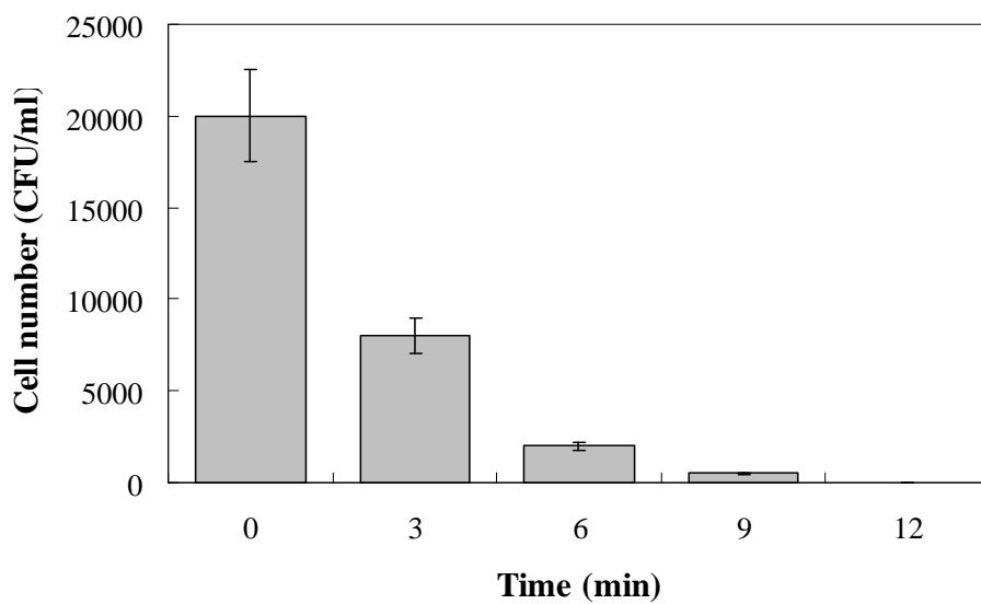
Figure 2. Bactericidal activity of S. mutans as a function of reaction time at propolis concentration 350 µg/ml.
