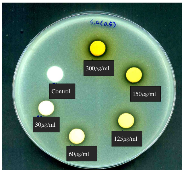
Figure 5. Clear zone of S. aureus as a function of propolis concentration.
