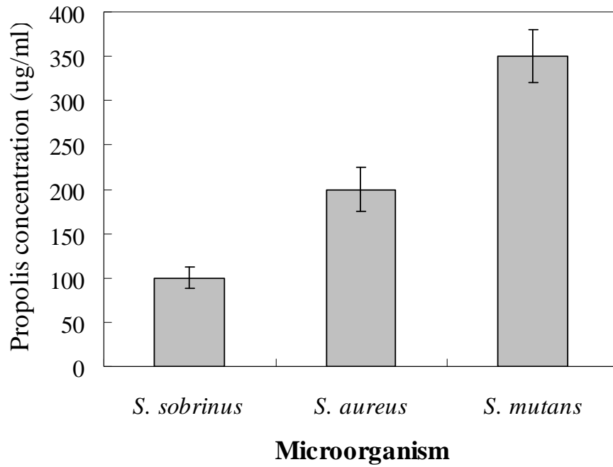
Figure 1. The MBC value of propolis at different microorganisms.
