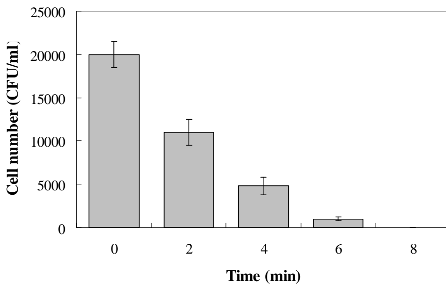
Figure 4. Bactericidal activity of S. aureus as a function of reaction time at propolis concentration 200 µg/ml.
