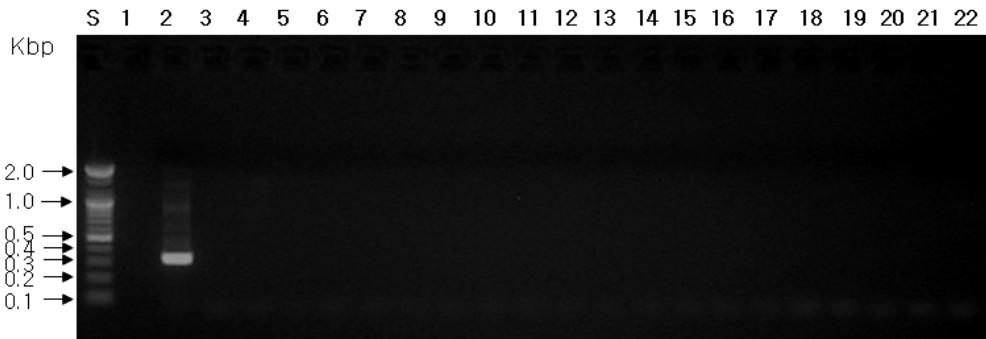
Fig. 9. Detection of T. denticola isolated from samples. The PCR products amplified with Ash-Td-F and Ash-Td-R primers. The PCR reactions were electrophoresed in 1.5% agarose gel. Lanes: S, 100 bp; 1, negative control (sterilized water); 2, T. denticola ATCC 35405 T ; 3-7, patient's No. 3; 8-12, No. 7; 13-17, No. 17; 18-22, No. 24.
