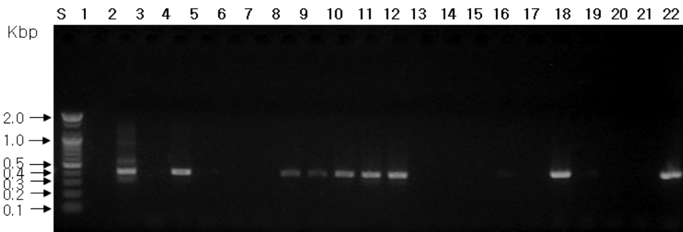
Fig. 10. Detection of Actinobacillus actinomycetemcomitans isolated from samples. The PCR products amplified with Ash-Td-F and Ash-Td-R primers. The PCR reactions were electrophoresed in 1.5% agarose gel. Lanes: S, 100 bp; 1, negative control (sterilized water); 2, A. actinomycetemcomitans ATCC 33384 T ; 3-7, patient's No. 3; 8-12, No. 7; 13-17, No. 17; 18-22, No. 24.
