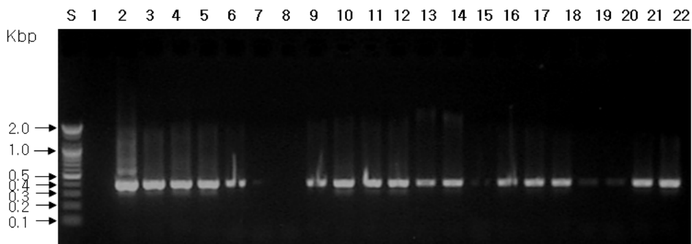
Fig. 6. Detection of P. gingivalis isolated from samples . The PCR products amplified with Ash-Pg-F and Ash-Pg-R primers. The PCR reactions were electrophoresed in 1.5% agarose gel. Lanes: S, 100 bp; 1, negative control (sterilized water); 2, P. gingivalis ATCC 33277 T ; 3-7, patient's No. 3; 8-12, No. 7; 13-17, No. 17; 18-22, No. 24.
