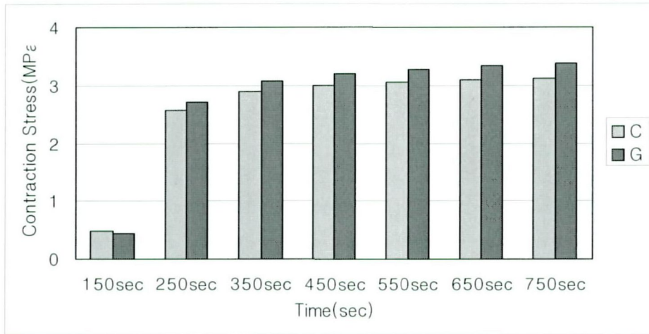
Fig. 6. Mean contraction stress values of compomer lining group C and G at each measuring point.
