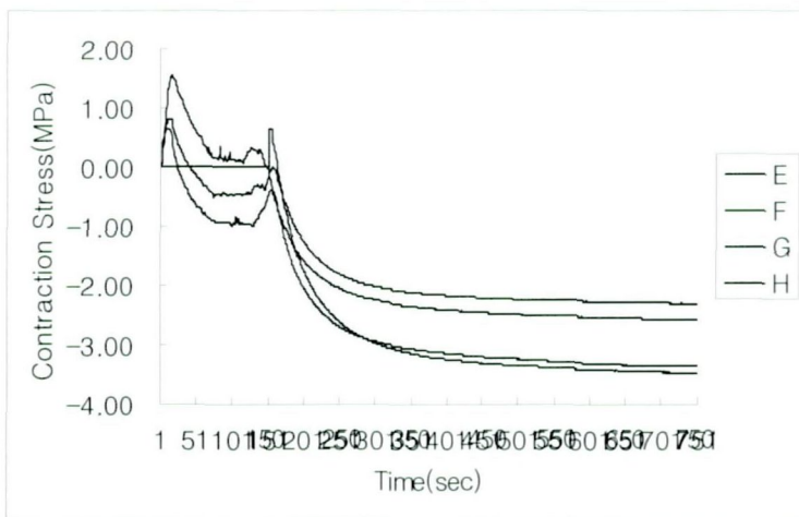
Fig. 4. Changes of contraction stress of each group cured with LED light during 750 seconds.
