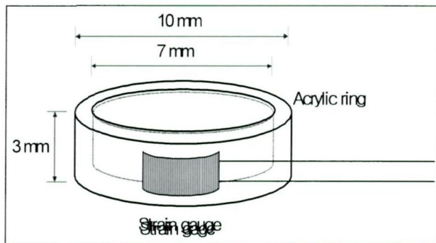
Fig. 2. Schematic drawing of strain gauge attached to acrylic mold for measuring of contraction stress.
