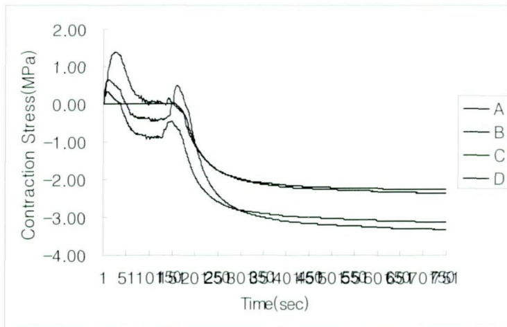
Fig. 3. Changes of contraction stress of each group cured with halogen light during 750 seconds.
