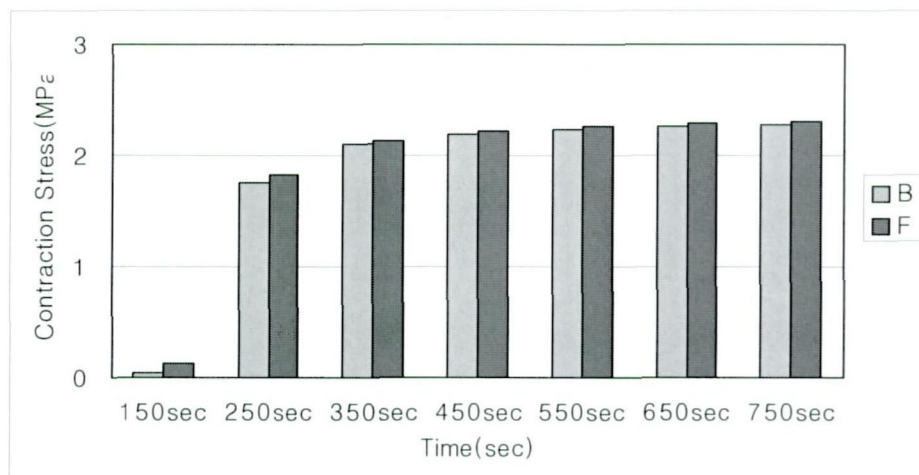
Fig. 5. Mean contraction stress values of flowable resin lining group B and F at each measuring point.
