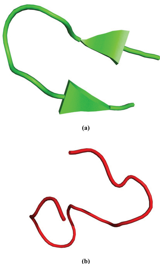
Fig. 1. Peptide structures selected (a) Kisspeptin-10, (b) Kisspeptin-15.
